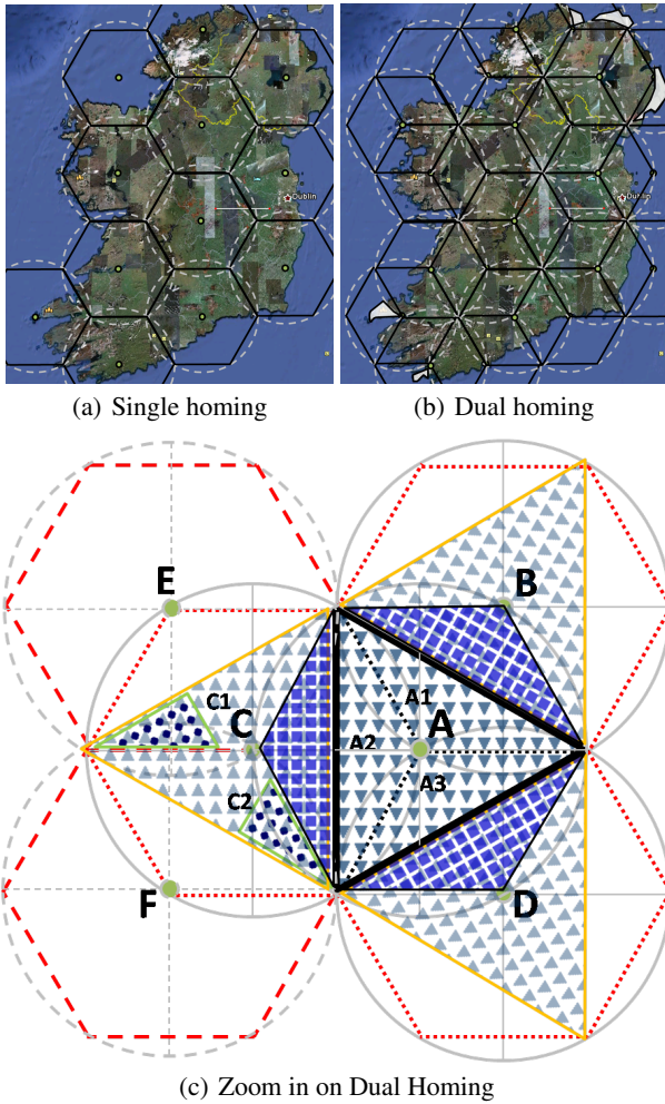
Figure 1: A geometric (honeycomb) model for designing resilient LR-PONs.
