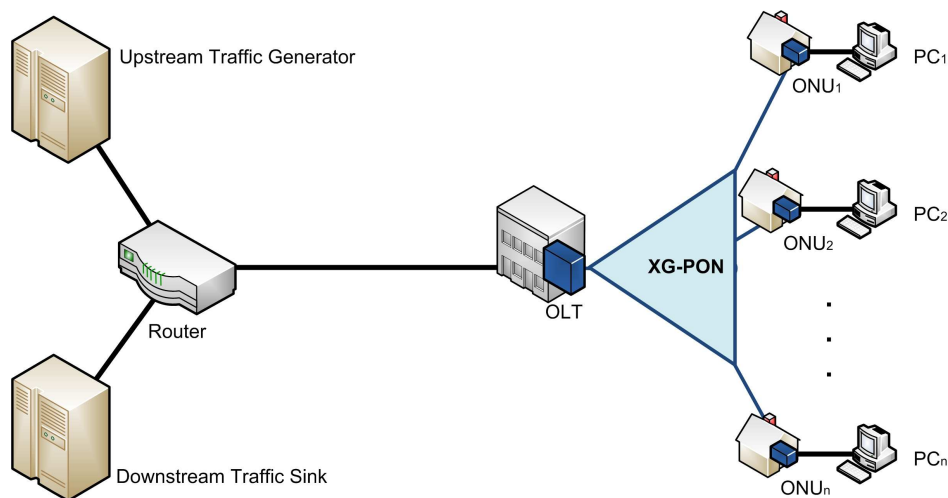
Fig. 11: Network Topology
