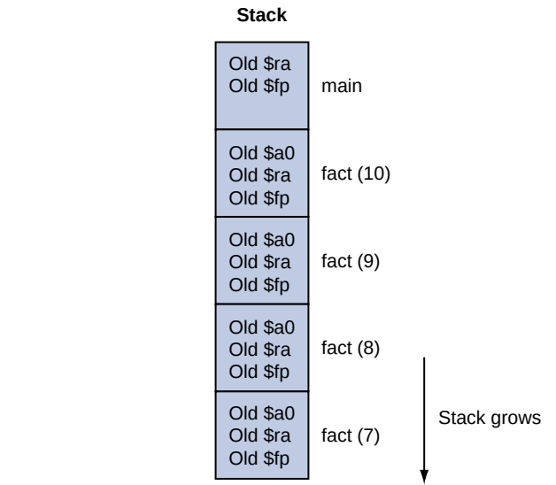
FIGURE A.6.3 Stack frames during the call of fact(7).
