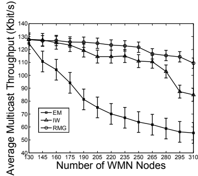
Fig. 12. The average throughput performance when the group size increases from 130 to 310.
