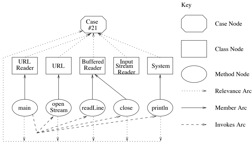
Figure 2: Semantic Net Fragment
