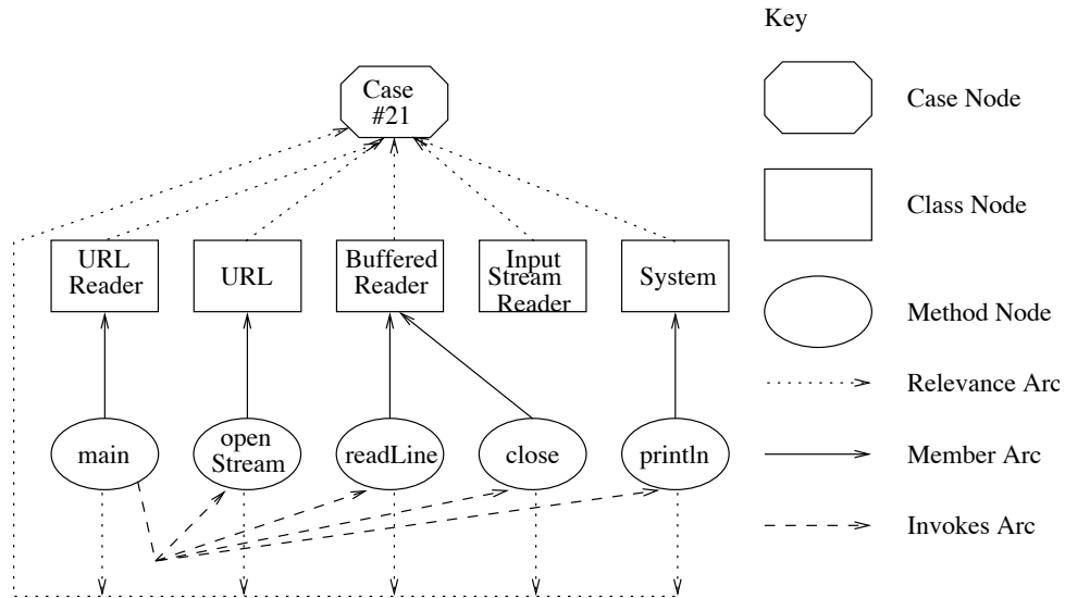
Figure 2: Semantic Net Fragment
