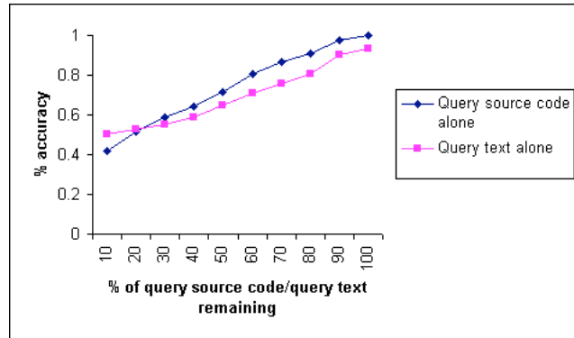
Figure 3: Accuracy for query source code/query text alone
